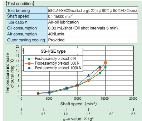
Fig. 9.25 relationship between preload and temperature increase
