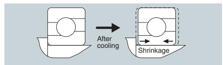
Fig. 6.6 Cooling after mounting by heating bearings
