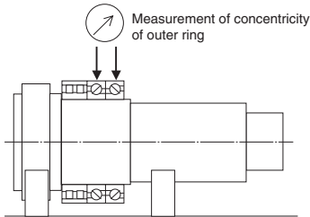
Fig. 11.1 Concentricity
