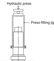
Fig. 6.1 Press-fitting pressure
