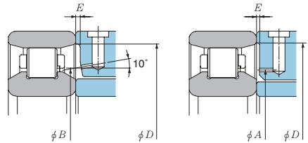
Fig. 7.7 N10HS type
