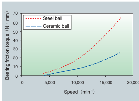
Fig. 9.19 Frictional torque
