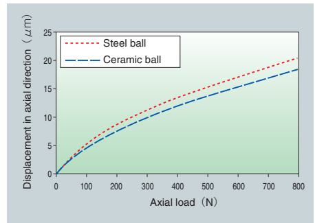
Fig. 9.20 Displacement in axial direction
