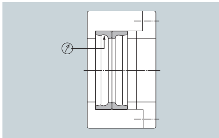
Fig. 6.13 Measuring position for roundness on outer ring raceway surface
