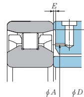
Fig. 7.8 N10HSR type
