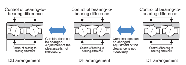
Fig. 9.14 Universal matching
