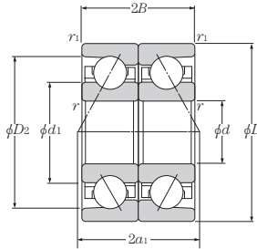
Back-to-back (DB)
