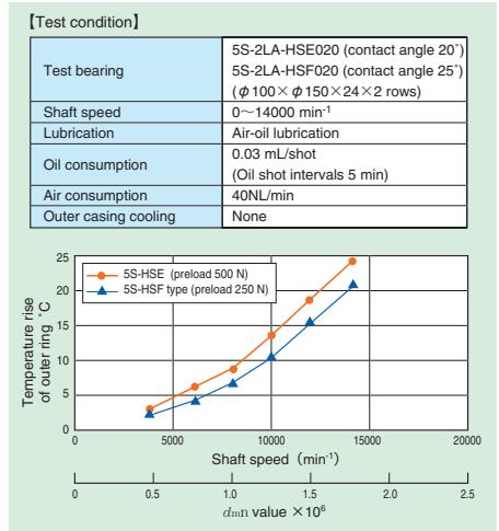
Fig. 9.28 Comparison of temperature rise
